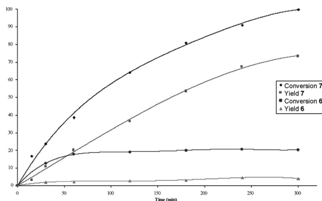
Figure 2. Kinetic curves of the Sonogashira-type coupling reaction depicted in Scheme 7 catalyzed by biminap and cationic bimionap complexes 6 and 7 , respectively; dodecane was used as an internal standard.
