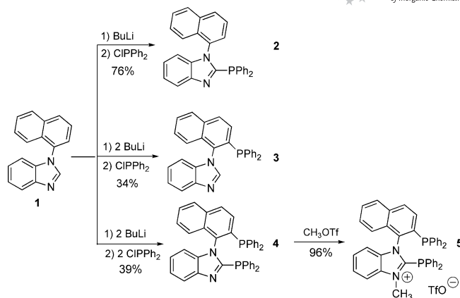
Scheme 3. Selective phosphanylation and methylation of the N -naphthylbenzimidazole core.
