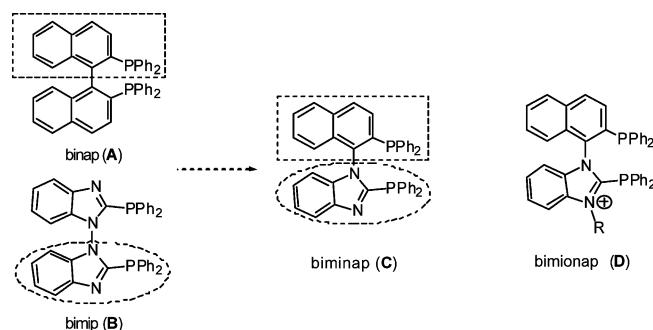
Scheme 1. Hybridization of the C_2 -symmetric binap ( A ) and bimip ( B ) ligands into the C_1 -symmetric bimnap ligand ( C ) and its bimionap iminium salt ( D ).
