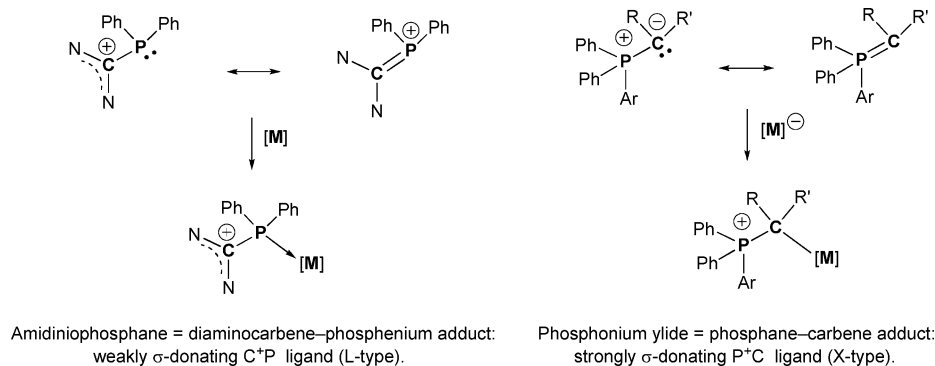
Scheme 2. Analogy between amidiniophosphane ligands (of the C^+P kind) and phosphonium ylide ligands (of the P^+C kind).
