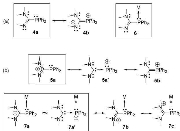
Scheme 5. (a) Resonance description of the imidazolylphosphane end of biminap in the free state ( 4 ) and the complexed state ( 6 ); (b) resonance description of the imidazolophosphane end of biminap in the free state ( 5 ) and the complexed state ( 7 ).
