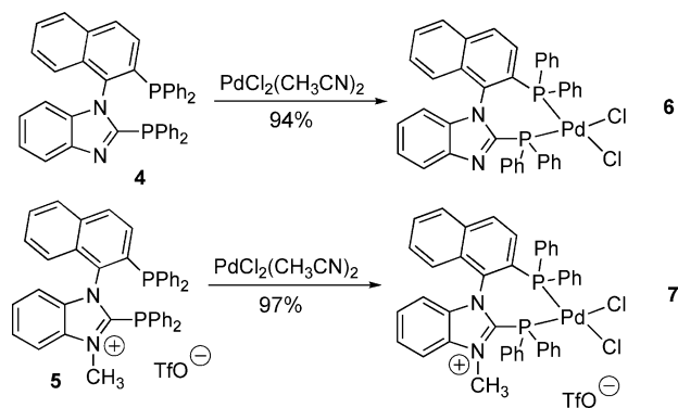
Scheme 4. Synthesis of isostructural \text{PdCl}_2 complexes of biminap 4 and biminap 5 .
