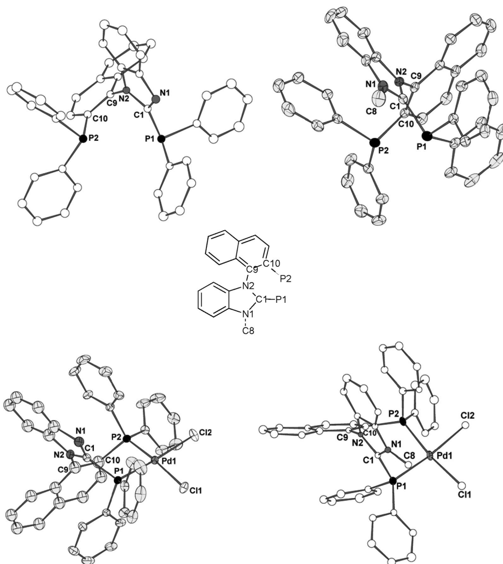
Figure 1. ORTEP views of the X-ray crystal structures of diphosphanes 4 (top left) and 5 (top right) and complexes 6 (bottom left) and 7 (bottom right) [with 30% probability for thermal ellipsoids of all non-hydrogen atoms in 5 and 6 . A common atom numbering scheme (centre) is adopted. All atoms were isotropically refined in 4 , and only Pd and P atoms were anisotropically refined in 7 . For representative bond lengths, see Table 1.
